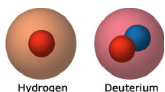
Figure 1. A hydrogen atom has only a single proton in its nucleus, whereas deuterium, a rarer isotope of hydrogen, has a proton and a neutron.
